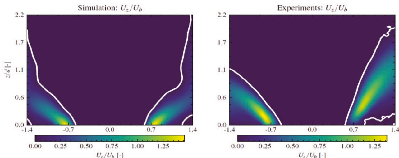
Figure 5.3: Comparison of non-dimensional mean axial velocity fields U_z : (left) preliminary LES cold-flow prediction scaled by bulk velocity U_b and (right) corresponding PIV measurements under identical conditions.
