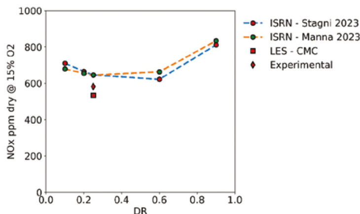
Figure 9.1: Comparison of NO x emissions for different chemical mechanisms for the cases with pressure 10 bar and primary zone equivalence ratio ( \phi_{pz} ) 1.5.
