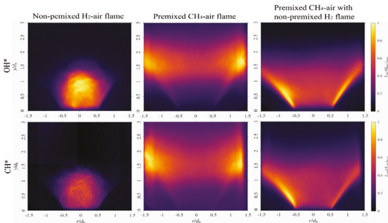
Figure 5.2: Normalised time averaged \text{OH}^* and \text{CH}^* chemiluminescence images of non-premixed \text{H}_2 -air flames, premixed \text{CH}_4 -air flames and premixed \text{CH}_4 -air with non-premixed \text{H}_2 flames. The equivalence ratio for premixed \text{CH}_4 -air flame is 0.8. The bulk velocity is maintained at 10 m/s for \text{CH}_4 flames and at 5 m/s for \text{H}_2 flames.
