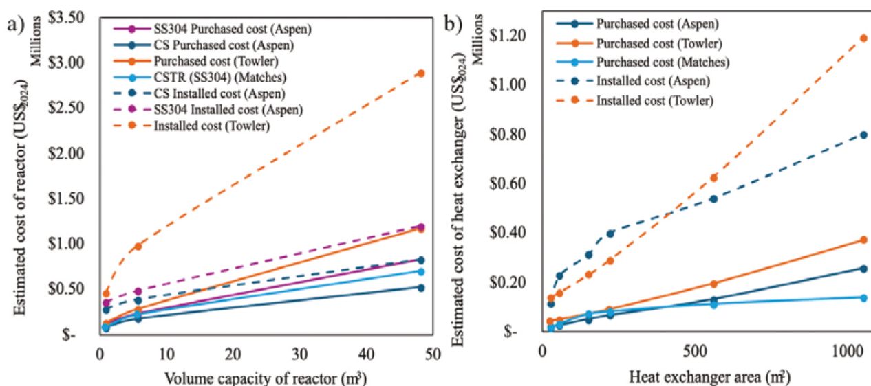
Figure 6.3: Comparison of the purchased and installed costs estimated from Aspen Plus, and the equipment cost calculating website Matches, for (a) a continuous stirred tank reactor and (b) a U-tube shell-and-tube heat exchanger.
