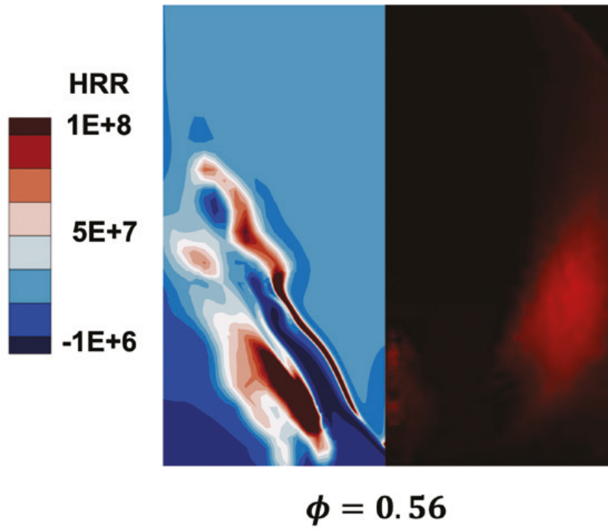
Figure 3.3: Comparison of heat release rate with the \text{OH}^* chemiluminescence image taken from Sidey and Mastorakos 2018.
