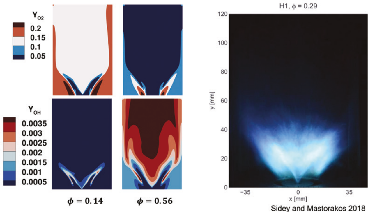
Figure 3.2: Comparison of species mass fractions for premixed equivalence ratio ( \phi_{\text{premixed}} ) of 0.14 and 0.56. Comparison is shown with the pure n-heptane flame by experiments of Sidey and Mastorakos 2018.
