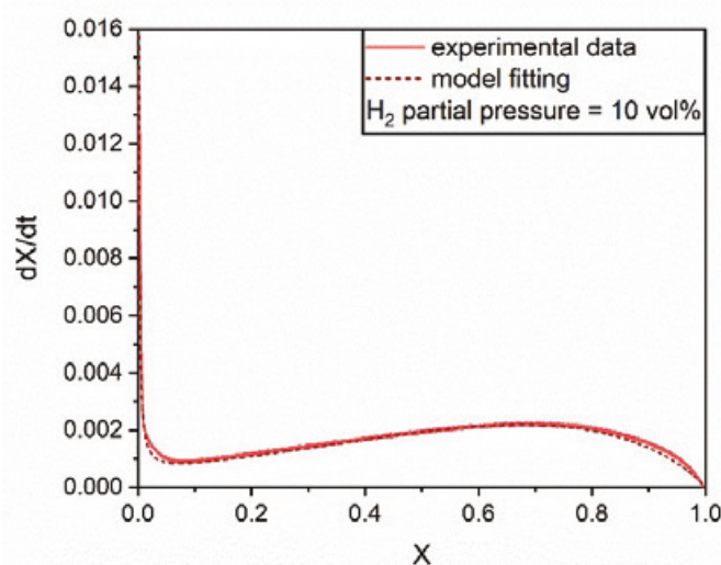
Figure 1.2: Overall reaction model fitting for the hydrogenation of Ni/CaCO 3 DFMs during the ICCU-Methanation cycles, in 10 vol% H 2 /N 2 at 400 °C.
