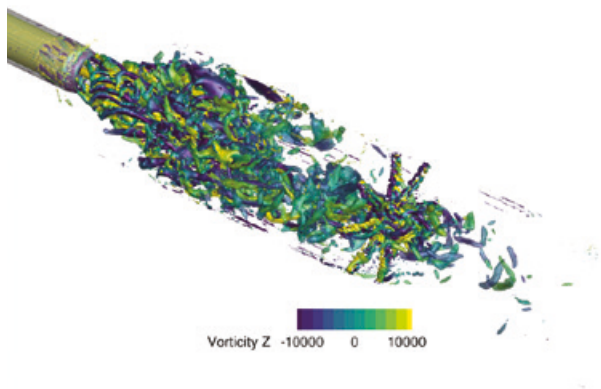
Figure 9.4: Iso-surfaces of Q-criterion for the anchor point LES-CMC simulation with decomposition ratio (DR) 0.5, primary zone equivalence ratio ( \phi_{pz} ) 1.0, and power 50.2 kW. The iso-surfaces are coloured by the z- vorticity.
