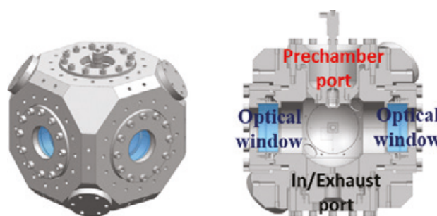
Figure 5.5: Schematic diagram of the high-pressure optical constant volume combustion chamber.
